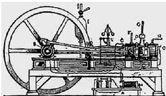
The Lenoir Gas Engine
